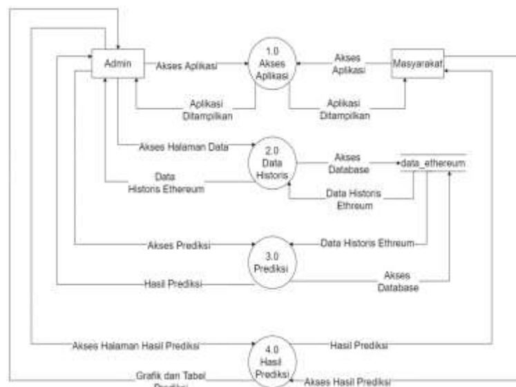
Image 4. DFD level 1
