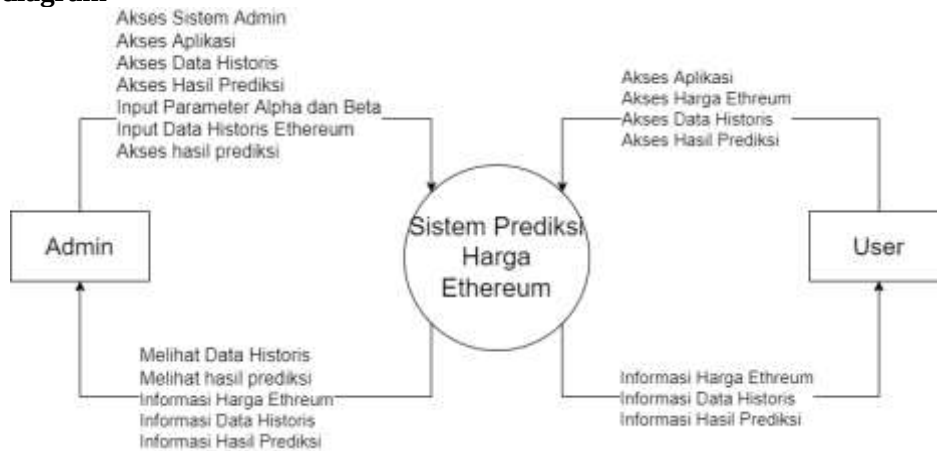
Image 3. Context diagram
